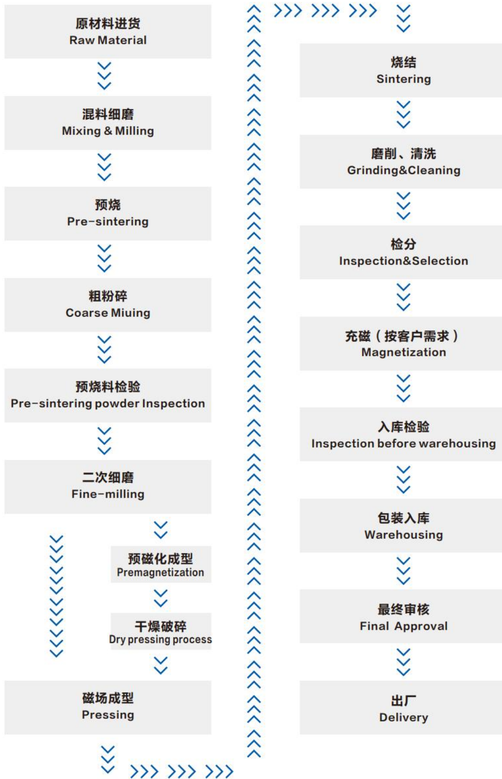
Hard Ferrite Process Flow Chart
